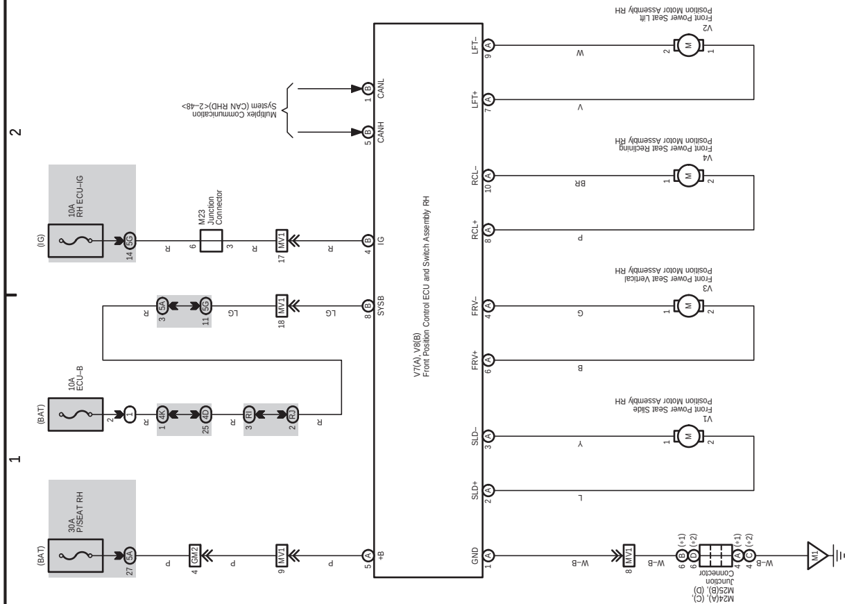
Power Seat (RHD Driver's Seat)
